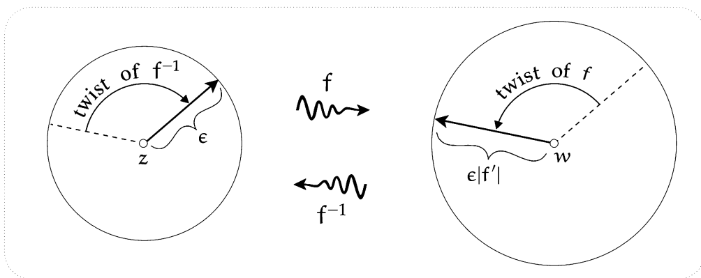
[5.8] The amplitwist of the inverse of an analytic mapping has the opposite twist and the reciprocal amplification, and so we obtain the familiar rule [f^{-1}(w)]' = 1/f'(z) .
