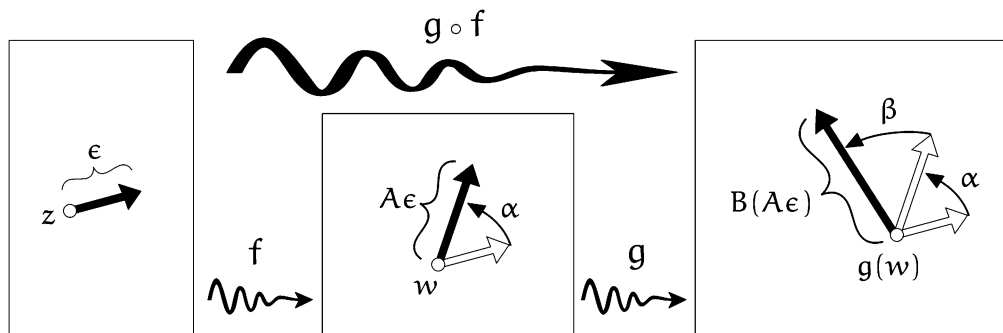
[5.7] Geometry of the Chain Rule. The local effect of the composition of two analytic mappings is an amplitwist that is the composition of their separate amplitwists, so we obtain the familiar chain rule.
