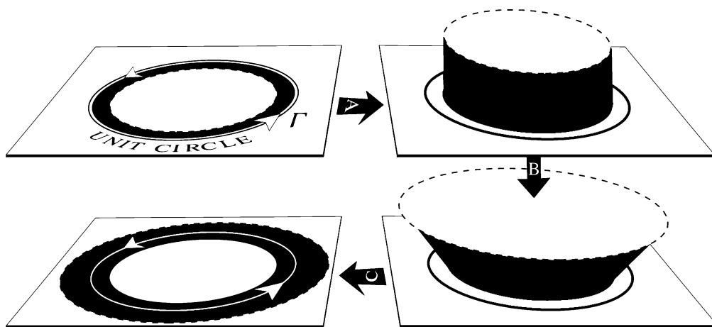
[7.13] (A) Form a “hat” by lifting up the part of the disc lying inside the dashed circle, some of the pastry dough outside the dashed circle being stretched to form the side of the cylinder. (B) Radially stretch the disc forming the top of this “hat” till its radius is greater than one. (C) Press down flat, i.e., project each point vertically down onto the plane. The final number of layers [bottom left] is indicated by the shading: one layer over the lightly shaded inner disc; two over the darkly shaded outer ring; and three over the black ring. You can now geometrically verify that (7.11) works in all three regions.
