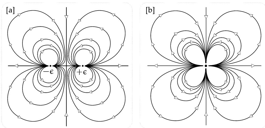
[11.15] The Quadrupole Pólya vector field (1/\bar{z}^3) . [a] Dipoles of strength \pm d at \pm\epsilon are merged by letting \epsilon \rightarrow 0 . But in order to form a quadrupole, the dipole moments d must grow in inverse proportion to the separation \epsilon , so that d\epsilon remains constant, otherwise the two opposite dipoles would simply annihilate each other, leaving no field. [b] The full phase portrait of the resulting quadrupole.
