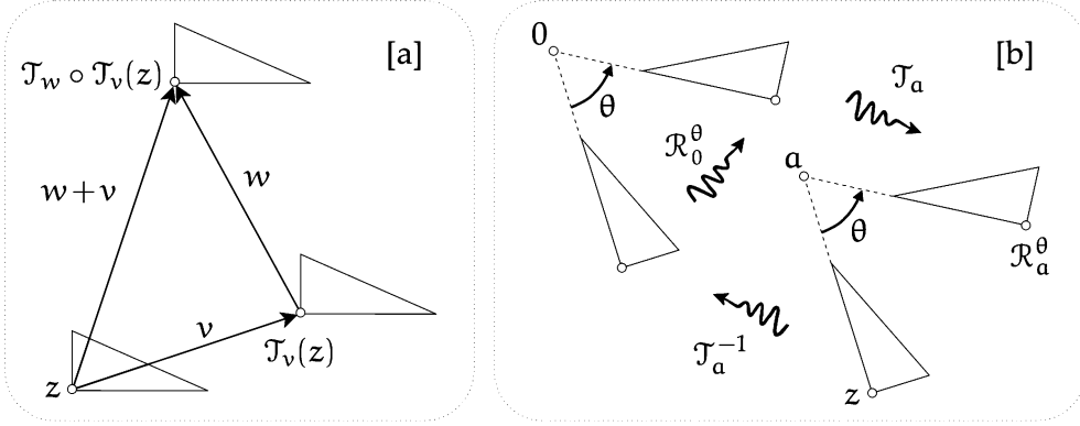
[1.13] Translations and rotations as complex functions. [a] Composition of translations is equivalent to addition: \mathcal{T}_w \circ \mathcal{T}_v(z) = \mathcal{T}_{w+v}(z) . [b] The general rotation \mathcal{R}_a^\theta can be performed by translating a to 0, rotating by \theta about 0, then translating 0 back to a .
