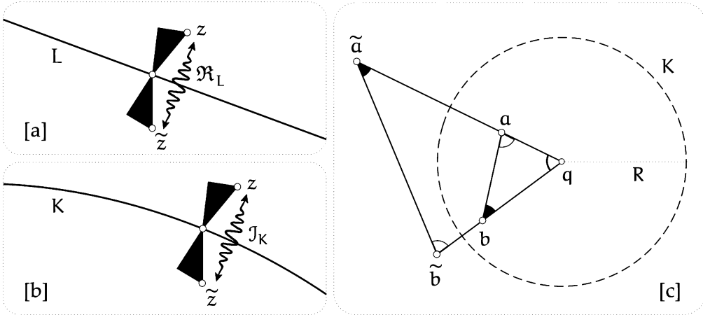
[3.2] [a] Ordinary reflection in a line. [b] If the radius of K is large, so that it starts to look straight, then geometric inversion z \mapsto \tilde{z} = \mathcal{J}_K(z) looks very much like ordinary reflection. More precisely, as z approaches K , then \mathcal{J}_K(z) is ultimately its reflection in the tangent to K . [c] Under inversion in K , the triangle aqb is similar to the triangle \tilde{a}\tilde{b}\tilde{q} .
