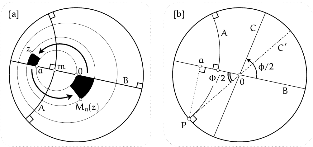
[6.39] Geometric interpretation and classification of the general Möbius automorphism, M_a^\phi . [a] The unique Möbius automorphism M_a = \mathcal{J}_B \circ \mathcal{J}_A that swaps a and 0 is the h-rotation \mathcal{R}_m^\pi through angle \pi about the h-midpoint m of the h-line segment 0a . [b] The most general Möbius automorphism is M_a^\phi = \mathcal{R}_0^\phi \circ \mathcal{R}_m^\pi = \mathcal{J}_C \circ \mathcal{J}_B \circ \mathcal{J}_B \circ \mathcal{J}_A = \mathcal{J}_C \circ \mathcal{J}_A . Thus M_a^\phi is an h-rotation, limit rotation, or h-translation according as A and C are intersecting, asymptotic, or ultra-parallel.
